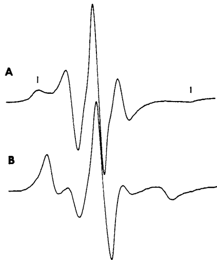
FIGURE 4 EPR spectra of FDNA-SL LC2 exchanged into glycerinated rabbit psoas muscle fibers bathed in rigor buffer. Spectrum A is oriented parallel to the magnetic field ( H_0 ) and spectrum B is oriented perpendicular ( H_0 ). The considerable difference in the line shape of the two spectra demonstrates that the probe is oriented with respect to the magnetic field and hence the fiber axis. The vertical lines indicate the approximately isotropic immobilized component seen in both spectra, that is thought to represent LC2 bound nonspecifically to the fiber.
