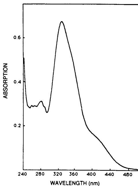
FIGURE 1 Absorption spectrum of 32 \mu\text{M} FDNA-SL LC2, containing 1 mol FDNA-SL bound per mole of LC2, in LC2 binding buffer, 1 cm pathlength. The maximum absorption of the fluoro-dinitroaniline ring at 330 nm is characteristic of binding to a sulfhydryl group rather than an amino group (two peaks at 345 and 425 nm) (Perkins et al., 1984).
